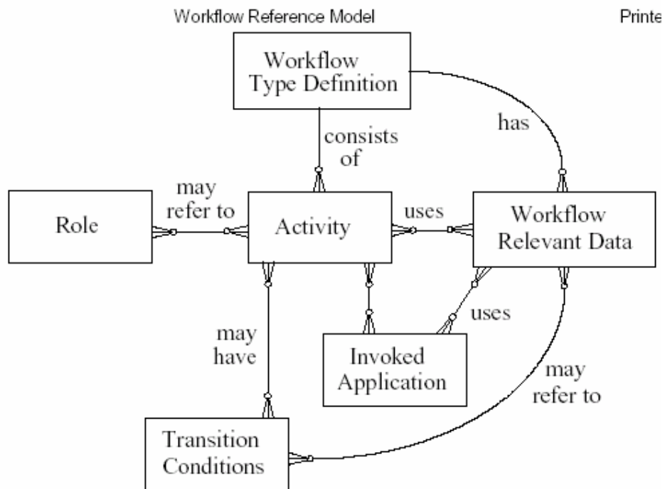
Fig 10 - Basic Process Definition Meta-model
